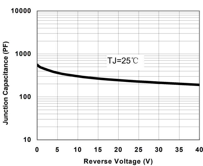
Fig.1-Typical Junction Capacitance
