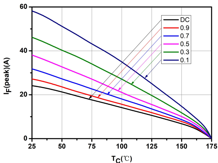
Fig.8-Current Derating
